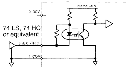
Figure 3. Equivalent Input Circuit for Operation with an Internal Power Supply
